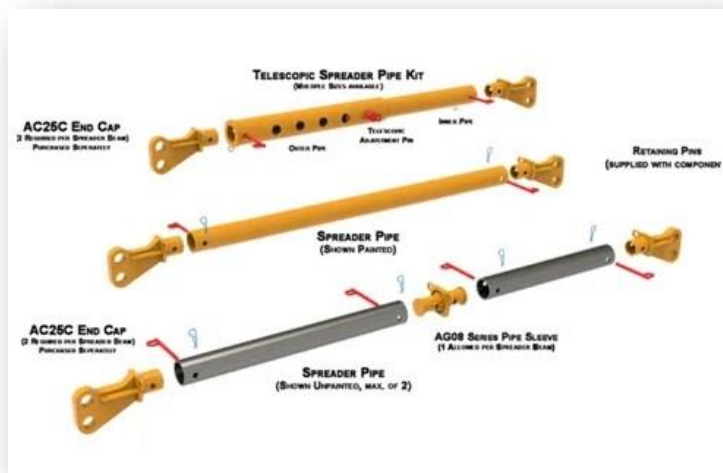
ADJUSTABLE TELESCOPE SPREADER BEAM
